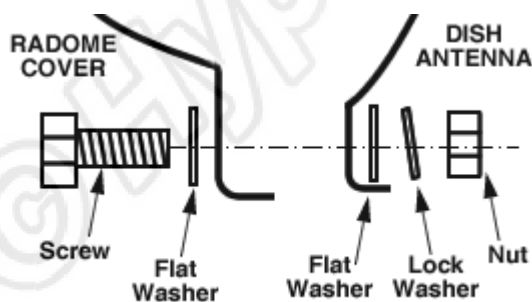
Assembly Detail
